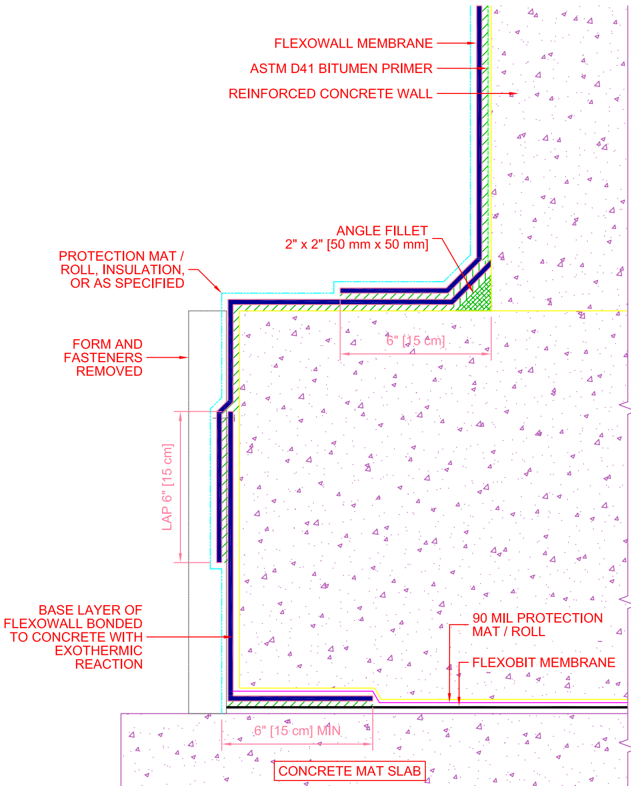
[STEP #2] TYPICAL FOUNDATION WITH REMOVABLE FORM BOARD
