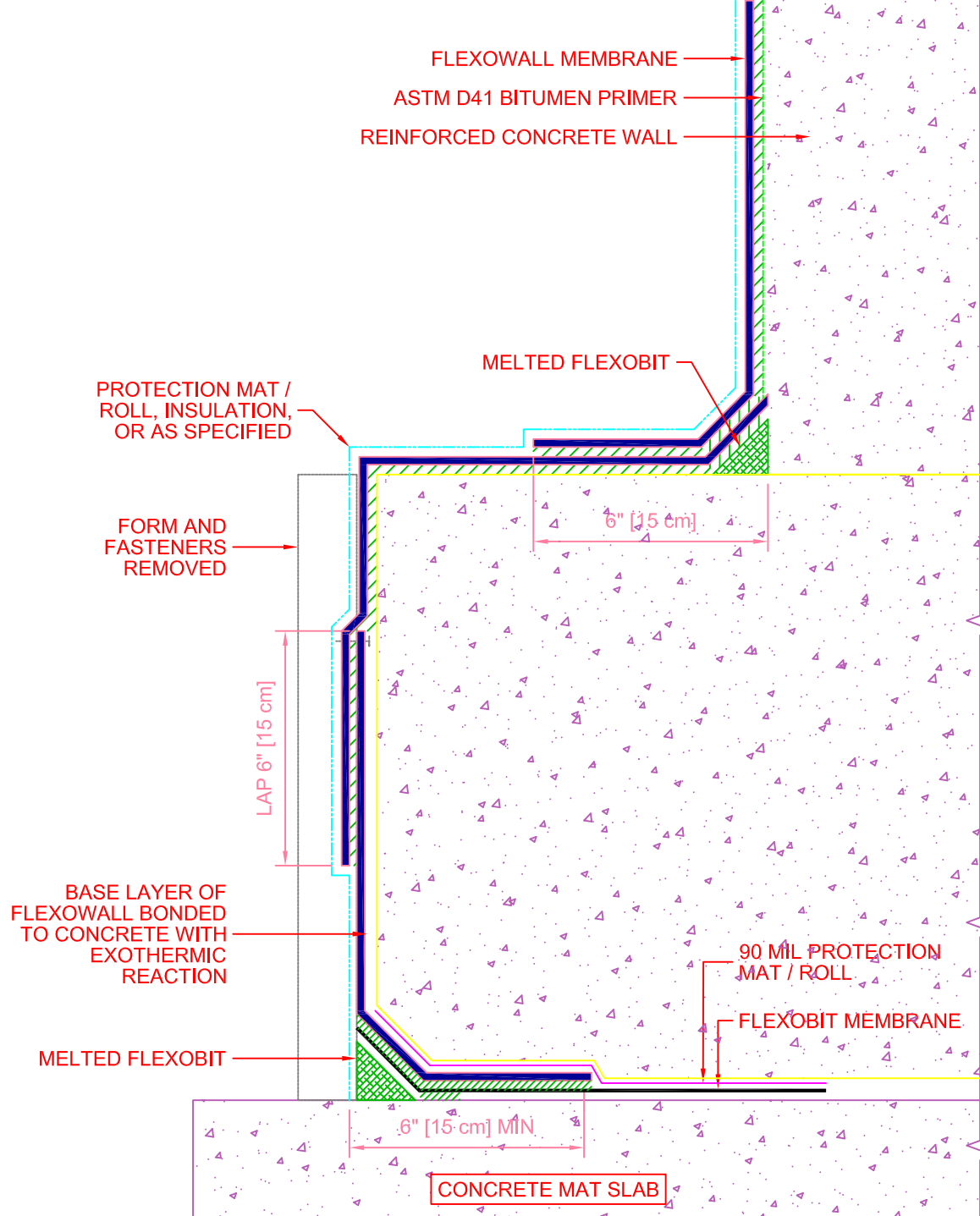
[STEP #2] TYPICAL FOUNDATION WITH REMOVABLE FORM BOARD
