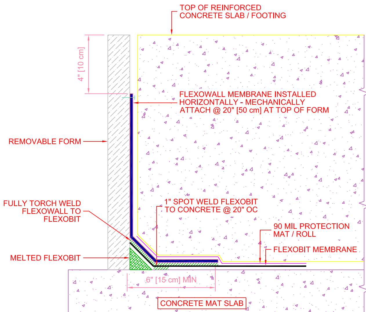
[STEP #1] TYPICAL FOUNDATION WITH REMOVABLE FORM BOARD
